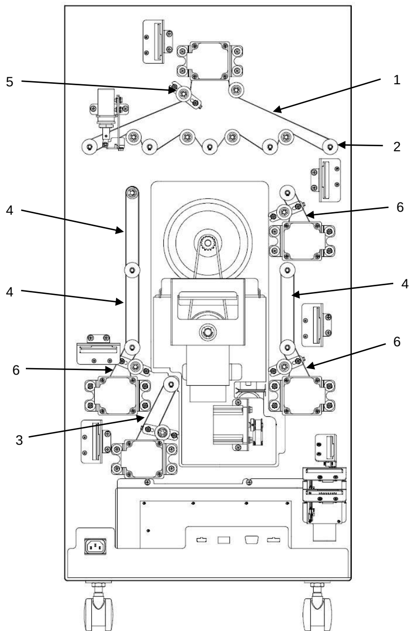
PL 2.9. Frame Assembly- Belts
