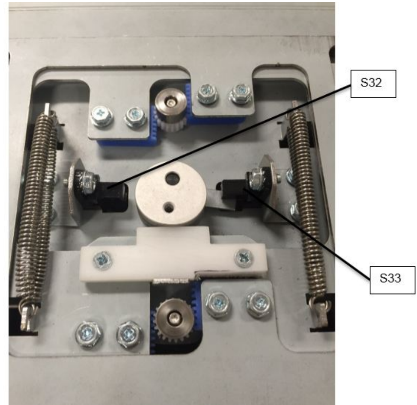
S32 and S33 are located on the Expanding T Module
