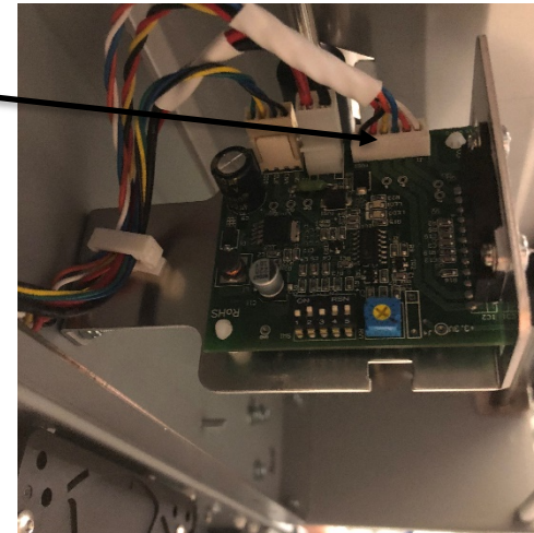
Motor Connector
