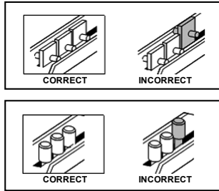
Figure 8.5 Pin Addition
