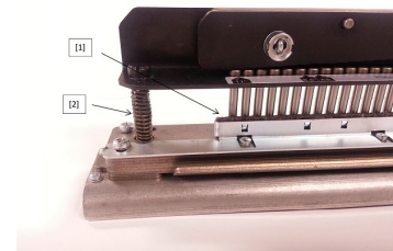
Figure 8.8 Lubrication
