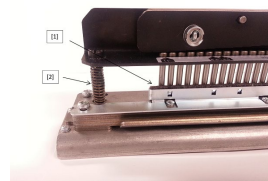
Figure 8.8 Lubrification
