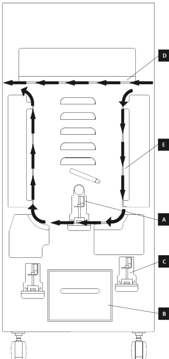
Paper flow and User Interactive sections of PUNCHalfa Plus
