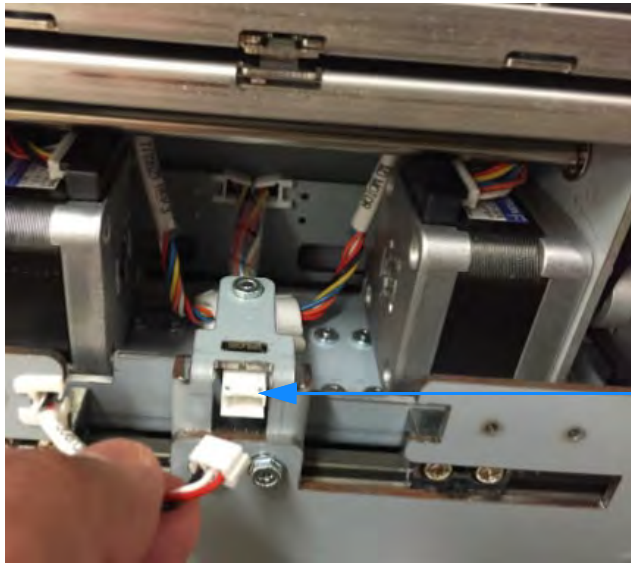
Connector
